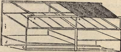
Fig. 37. Chauvière's Propagating-oven.
